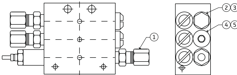
"b" Porting - Closure Plug & Clamping Ring
