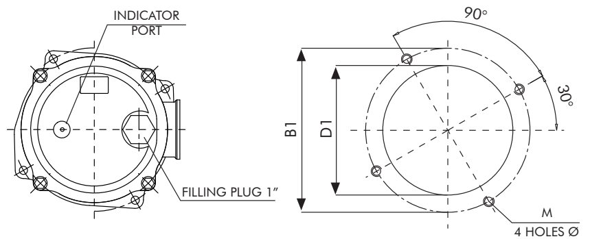
FR - 1 - 50 / 51 / 60 / 64 TANK MOUNTING PATTERN
