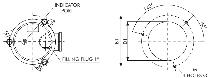
FR - 1 - 50 / 51 / 60 / 64 TANK MOUNTING PATTERN
