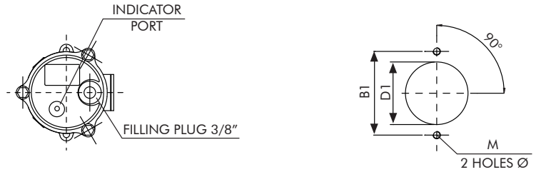
FR - 1 - 40 / 43 TANK MOUNTING PATTERN
